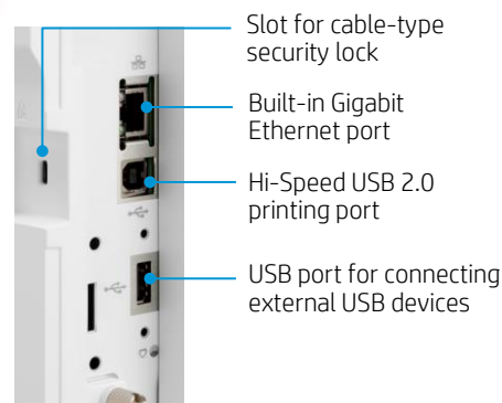
Rear I/O panel close-up
